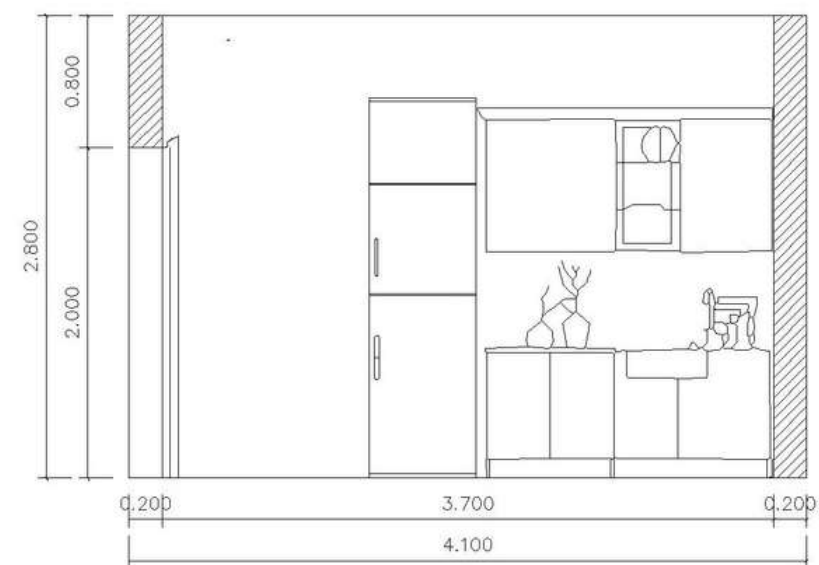
A Cuisine A Façade 1:50
