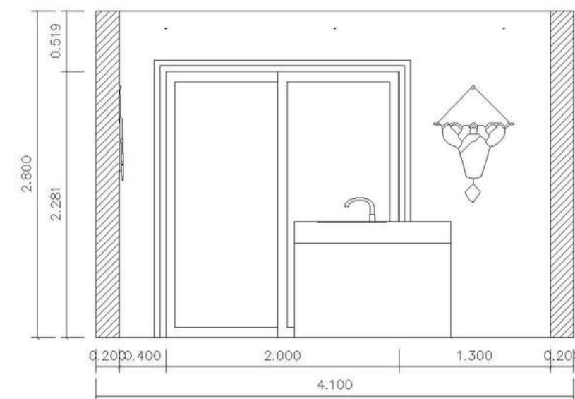
C Cuisine C Façade 1:50
