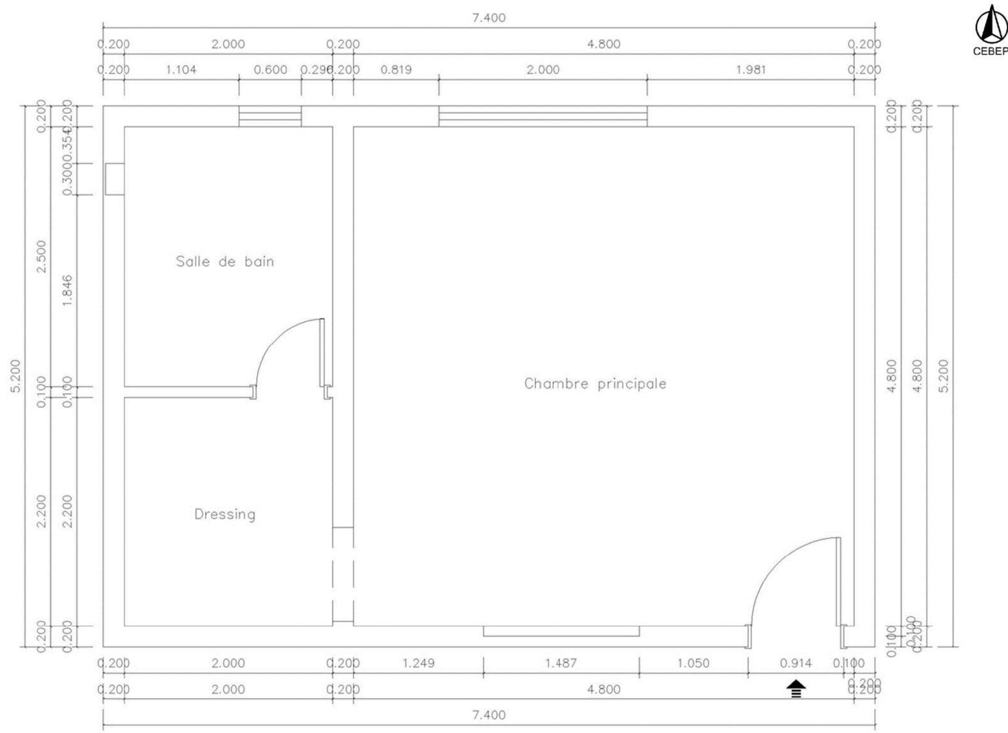
Plan Initial 1:50
